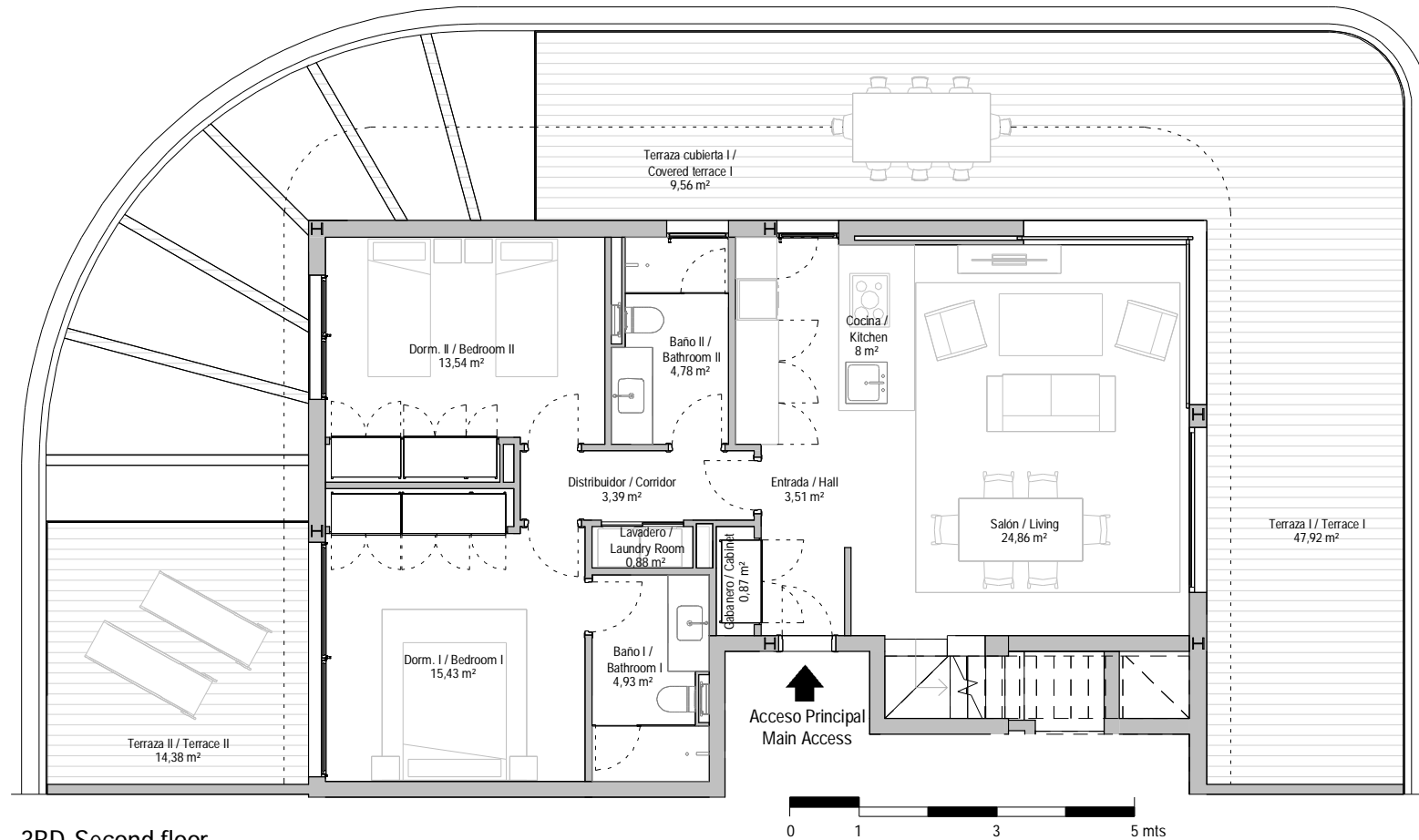
Terrace layout
